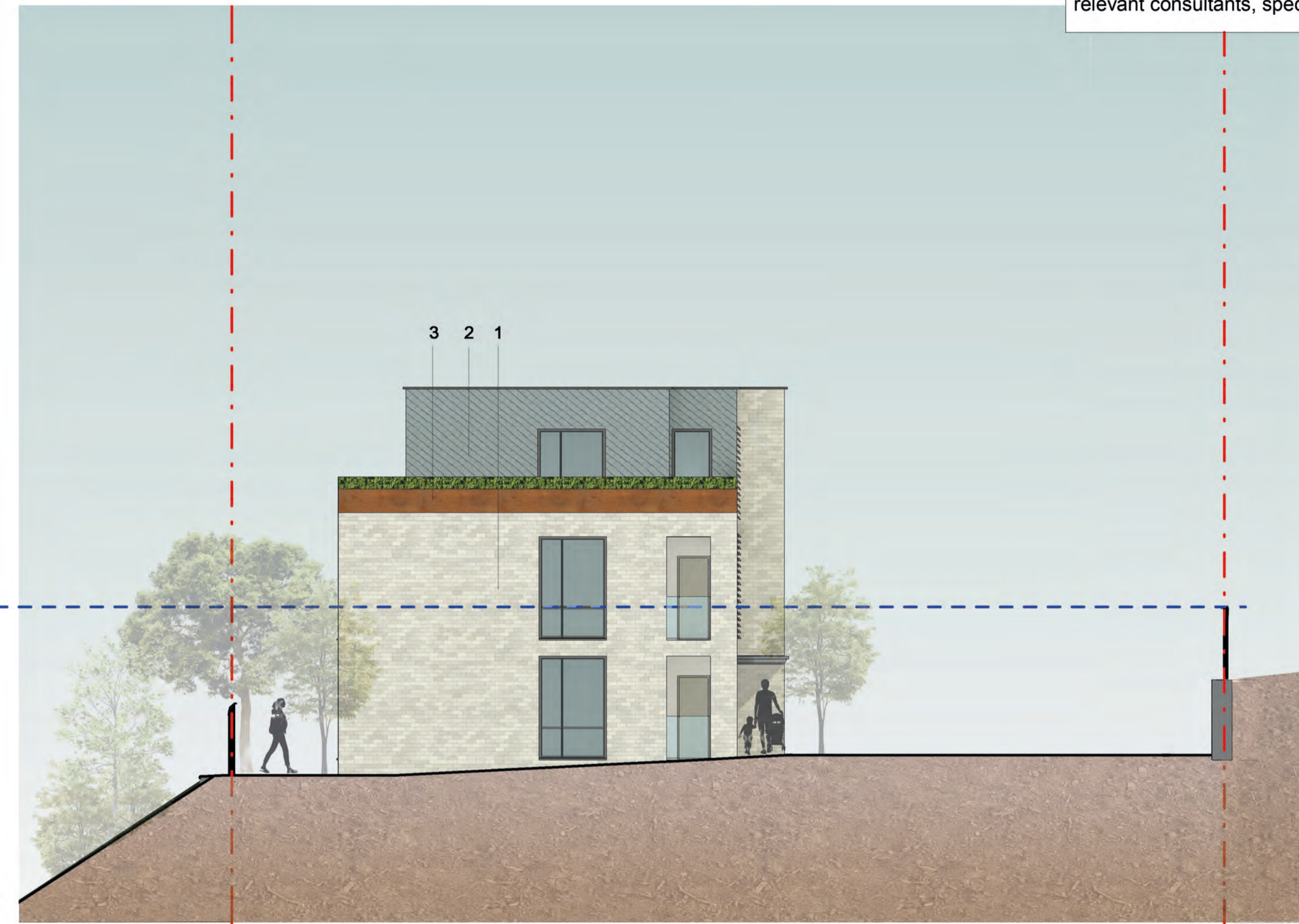
Block B South Elevation 1 : 100
